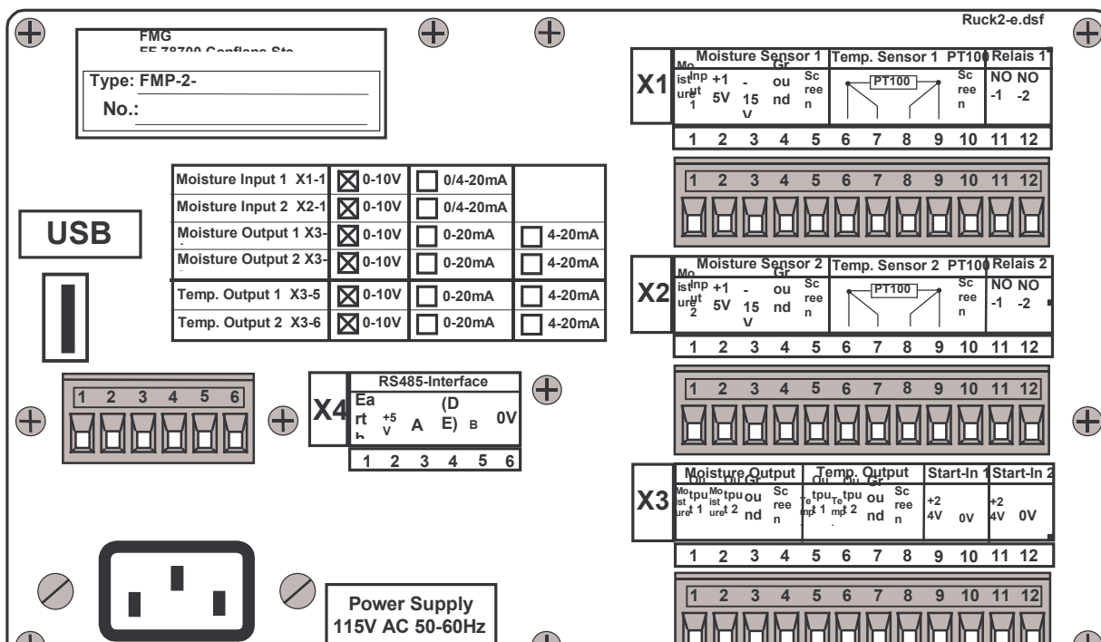
Backside of FMP-2: Two channel version, 115VAC mains, PT100-option
