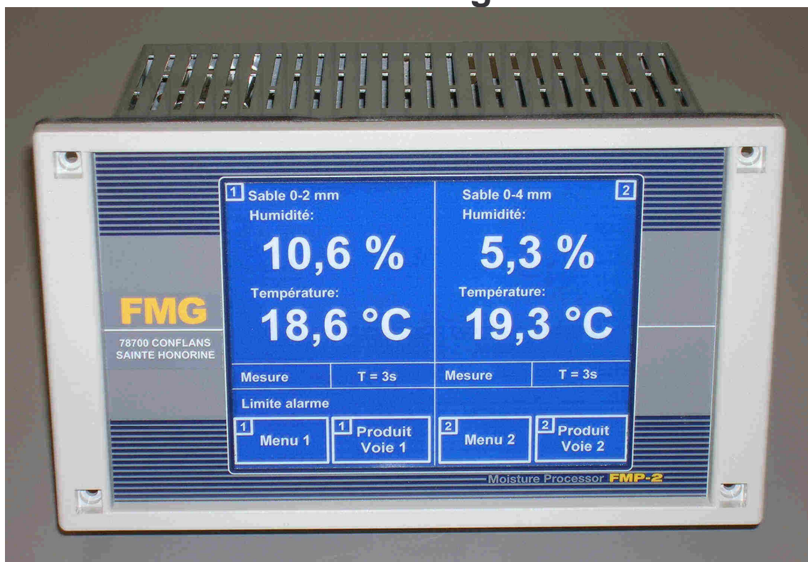
Figure 1: Moisture Processing Unit FMP-2 (two channel version)
