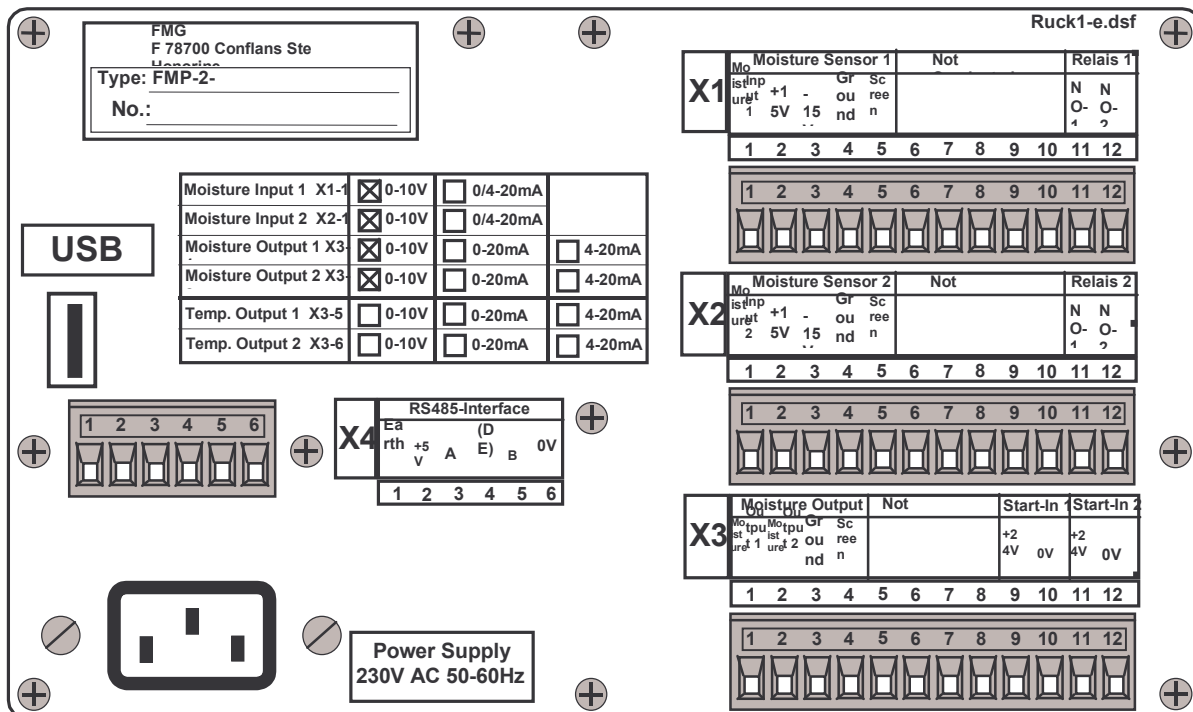
Backside of FMP-2: Two channel version, 230VAC mains, without PT100-option
