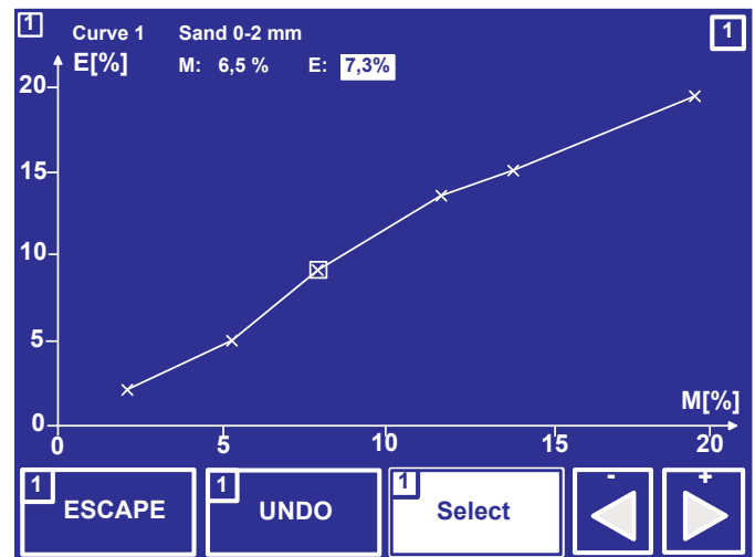
Figure 15: Editing of calibration point
